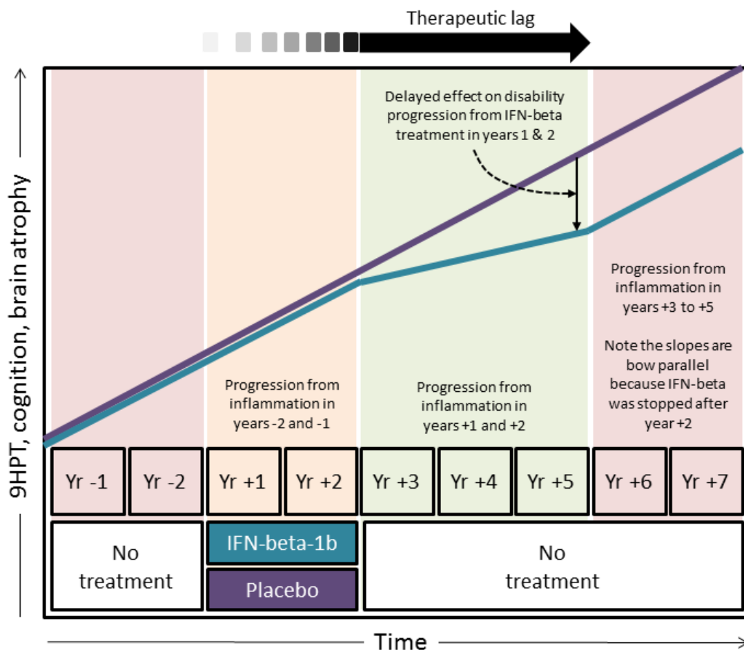
Figure 3: Therapeutic lag
