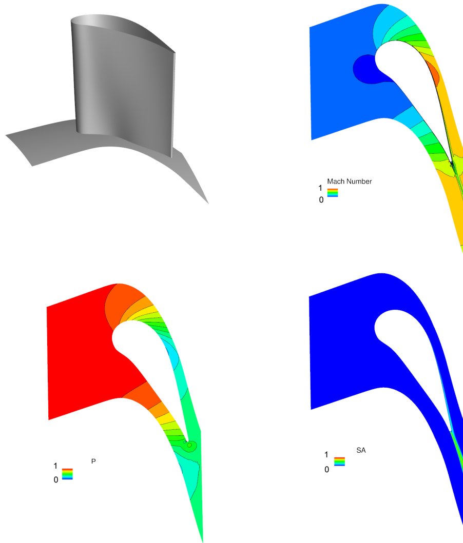
Figure 2: Case 1, Nozzle Guide Vane (NGV). Upper left: NGV geometry; upper right: Mach number contours at midspan; lower left: static pressure contours at midspan; lower right: Spalart-Allmaras turbulence variable contours at midspan. All legends are non-dimensionalised using their corresponding minimum and maximum values.
