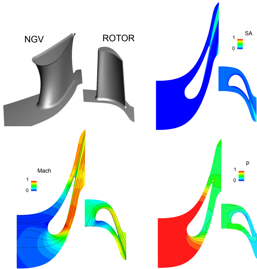
Figure 7: Case 3, NGV + rotor with tip gap. Upper left: NGV and rotor geometry; upper right: SA variable contour; lower left: Mach contour with 2-D streamline; lower right: static pressure contour. The contour plots are taken at midspan. All legends are non-dimensionalised using their corresponding minima and maxima.
