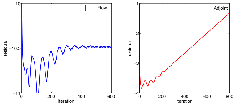
Figure 8: Case 3: convergence history of both Block-Jacobi flow and adjoint solvers.
