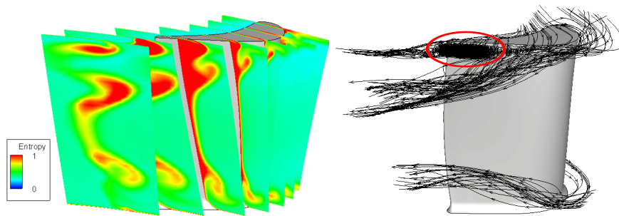
Figure 9: Case 3, flow visualisation around the rotor. Left: entropy contour plot at various axial locations; right: streamline illustrating the tip vortex and the two passage vortices.
