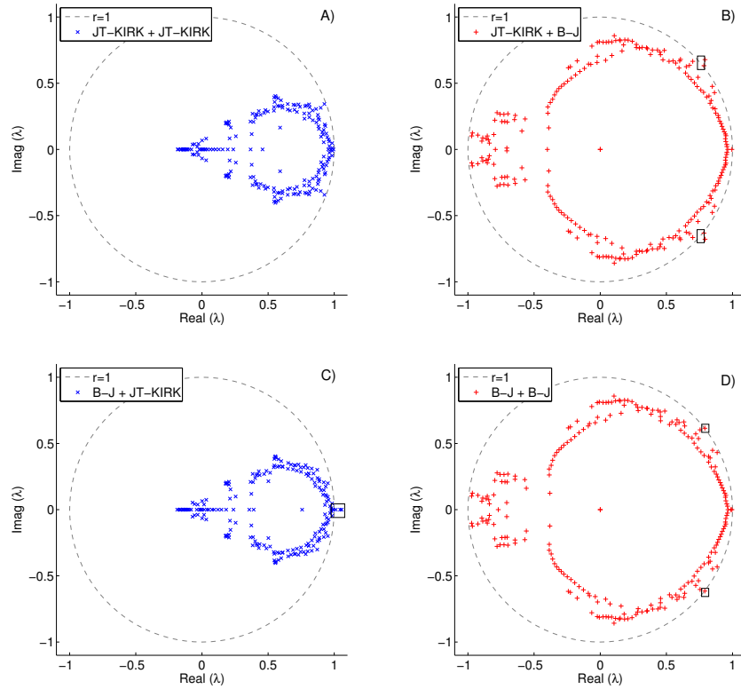
Figure 15: The eigenvalues for the solver combinations of Tab. 10. Outlying eigenvalues with |\lambda| > 1 are highlighted in boxes.
