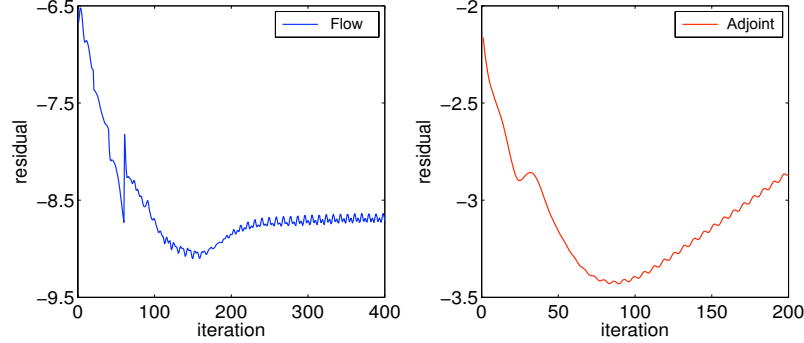
Figure 12: Case 4, LCO convergence of the flow solver and the divergence of the adjoint solver.
