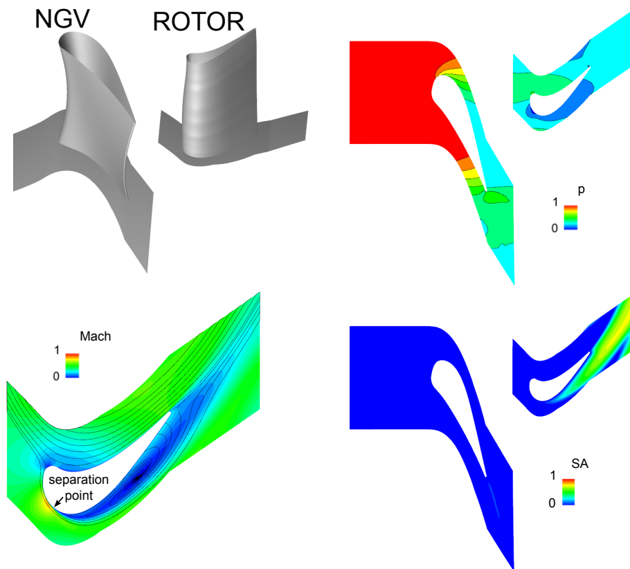
Figure 11: Case 4, NGV and skewed rotor. Upper left: NGV and rotor geometry; upper right: static pressure contour; lower left: Mach contour with 2-D streamline for the rotor only; lower right: SA variable contour. The contour plots are taken at midspan. All legends are non-dimensionalised using their corresponding minima and maxima.
