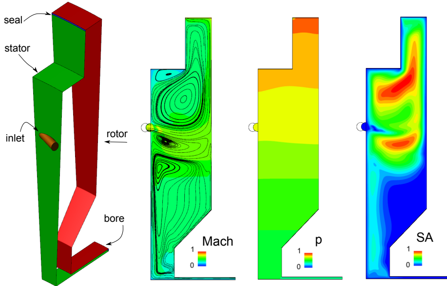
Figure 6: Case 2, cavity. From left to right: (1) cavity geometry, (2) Mach contours with 2-D streamline, (3) static pressure contours and (4) SA variable contours. Contour plots are taken at the medium azimuthal angle. All legends are non-dimensionalised using their corresponding minimum and maximum values.
