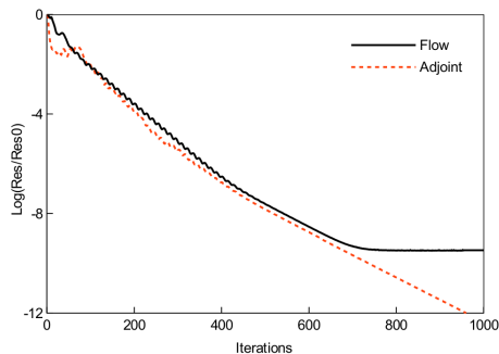
Figure 10: Case 3: convergence history of flow and adjoint solvers using JT-KIRK algorithm.
