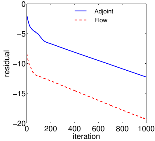
Figure 13: Case 4: convergence history of both JT-KIRK flow and adjoint solvers.
