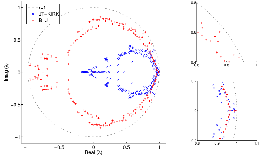
Figure 14: The dominant eigenvalues values for both the B-J and JT-KIRK solvers produced using Arnoldi iterations. The zoomed region on the top right show the unstable mode.
