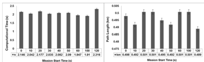
Fig. 10. Comparison of computational time and path length obtained with different mission start time (a) 0 (b) 10 (c) 20 (d) 30 (e) 40 (f)50 (g) 60 (h) 100 (i) 120 seconds.
