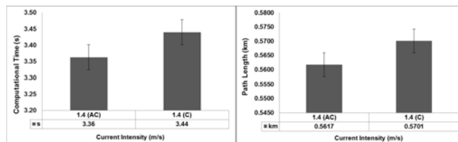
Fig. 12. Comparison of computational time and path lengths obtained for currents moving with intensity of 1.4 m/s in anti-clockwise (AC) and clockwise (C) direction.
