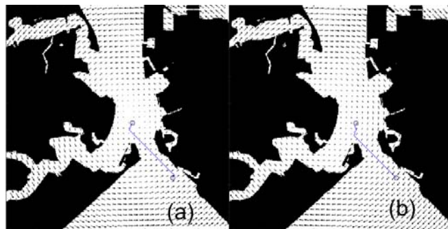
Fig. 11. Comparison of paths obtained for currents moving with intensity of 1.4 m/s in (a) anti-clockwise and (b) clockwise direction.
