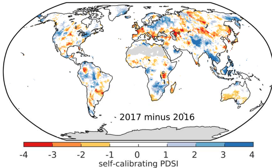
FIG. Z. Change in drought from 2016 to 2017 (mean scPDSI for 2017 minus mean scPDSI for 2016). Increases in drought severity are indicated by negative values (yellow-red), decreases by positive values (pale-dark blue). No calculation is made where a drought index is meaningless (grey areas: ice sheets or deserts with approximately zero mean precipitation).
