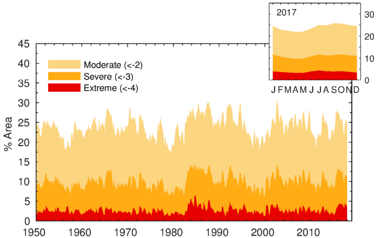
FIG. Y. Percentage of global land area (excluding ice sheets and deserts) with scPDSI indicating moderate (<-2), severe (<-3) and extreme (<-4) drought for each month of 1950–2017. Inset: each month of 2017.
