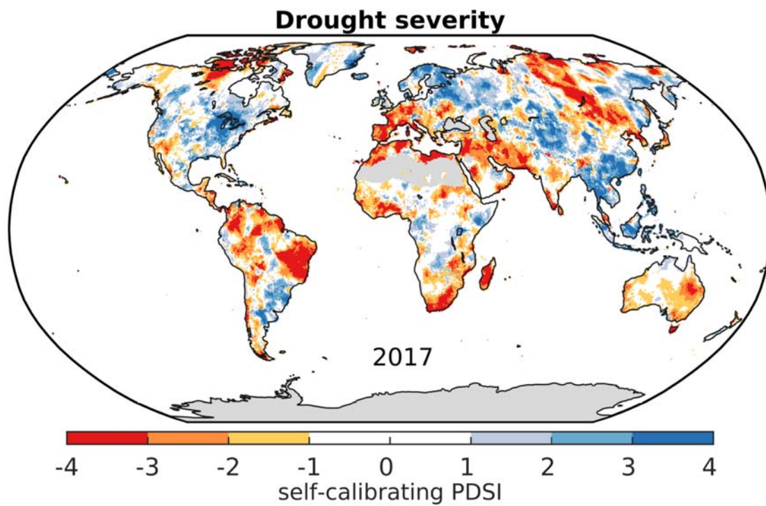
PLATE X. Mean scPDSI for 2017. Droughts are indicated by negative values (yellow-red), wet episodes by positive values (pale-dark blue). No calculation is made where a drought index is meaningless (grey areas: ice sheets or deserts with approximately zero mean precipitation).
