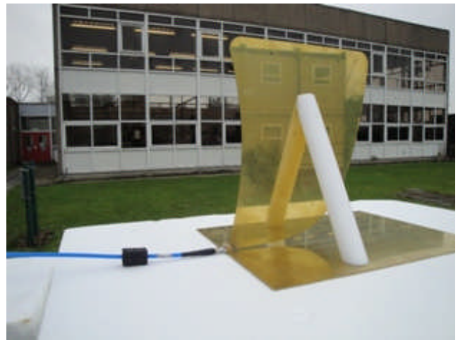
Fig. 8. Free space measurement on an OATS.
