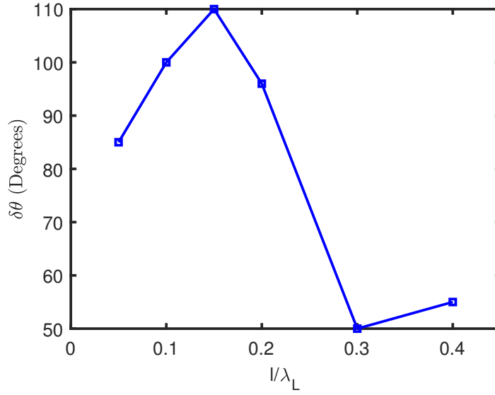
Figure 3. Variation of the second average emission angle, \delta\theta , with target thickness. This angle provides information on the partition of the RR force into the longitudinal and transverse directions.
