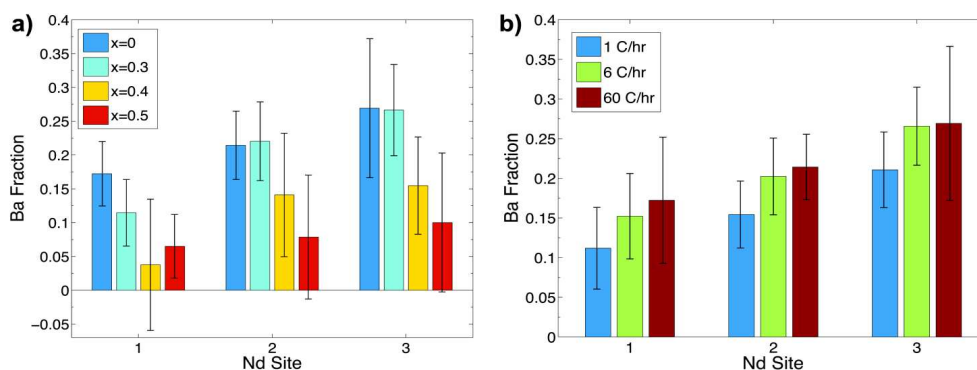
Figure 10. Plots of the fraction of Ba on Nd columns for different samples. The error bars represent one standard deviation and represent the random variation found within the area sampled in each case: a) the dependence of Ba partitioning to the 3 column types as a function of composition, n , in the formula, Ba_{6-3n}Nd_{8+2n}Ti_{18}O_{54} ; b) the dependence of Ba partitioning on cooling rate for the n=0 sample.
