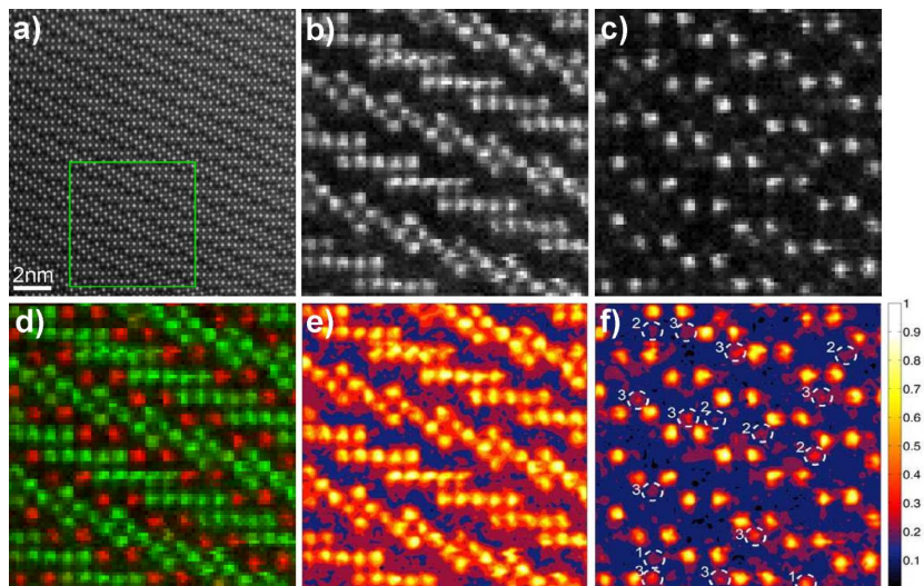
Figure 9. a) [010] HAADF STEM survey image of the n=0 sample cooled at 1^{\circ}\text{C/hr} . Atomic-resolution EELS maps of b) Nd M_{4,5} and c) Ba M_{4,5} and d) RGB overlay of raw Nd and Ba maps (in green and red, respectively); e) and f) normalised Nd M_{4,5} and Ba M_{4,5} maps, respectively, plotted after processing using the procedure for internal intensity normalization described in the methods section. Note the significant number of locations in the Barium map where significant intensity is found on Nd positions (ringed). Both b) and c) are shown on the same calibrated colour scale shown on the far right on a 0-1 scale, where 0 represents none of an element, and 1 represents the maximum intensity in the map.
