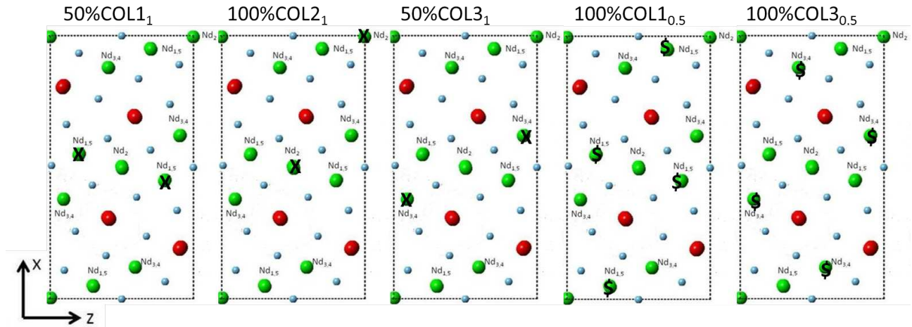
Figure 2. [010] projection of the \text{Ba}_{6-3n}\text{Nd}_{8+2n}\text{Ti}_{18}\text{O}_{54} ( n=0 ). Five configurations were studied using DFT with different substitution of Ba in tetragonal columns. \text{Nd}[3]/[4] , \text{Nd}[1]/[5] and \text{Nd}_2 represent Nd sites of tetragonal column 3, 1 and 2 respectively. X and $ signs represent 100% and 50% substitution of Ba on Nd sites. Green Nd, Red Ba and Blue Ti. X and Z directions represent the a and c lattice parameters.
