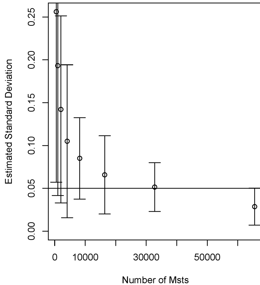
Fig 2. Convergence of MMST creation. (see also [41])
