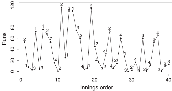
Fig. 1. Innings played by Ian Bell against Australia between 2009 and 2015: \blacktriangle , \triangle , away matches; \triangle , \circ , not-out innings; 1–4, innings number
