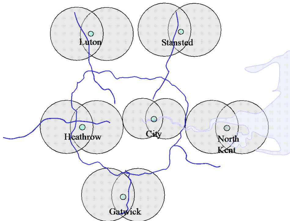
Figure 12: Airspace Design Footprints for five existing airports and a new airport in North Kent.
