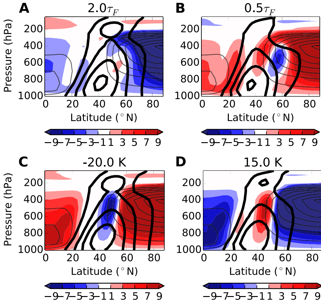
FIG. 7. Time-mean local APE [calculated using Eq. (6)] responses. The thin black contours show the absolute values of the control run (starting at 5 \times 10^5 \text{ J kg}^{-1} in the midlatitudes with intervals of 5 \times 10^5 \text{ J kg}^{-1} ). The color shading shows the anomalies from the control run of the extreme cases of the reference runs, viz., showing the runs of (a) lowest and (b) highest eddy friction and the (c) highest and (d) lowest polar cooling. Units are 10^4 \text{ J kg}^{-1} . The absolute values of the heat flux field are also shown in the thick black contours (starting at 5 \text{ K m s}^{-1} with intervals of 5 \text{ K m s}^{-1} ).
