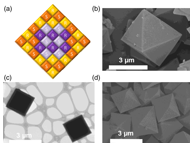
Figure 2. (a) General scheme showing the structure of a core-shell multicomponent heterochiral cage cocrystals (core = purple/mauve; shell = yellow/orange). (b) SEM image of a large CC3-RScore/CC19-RShell crystal. (c-d) TEM and SEM images of large CC19-RScore/CC3-RShell crystals.
