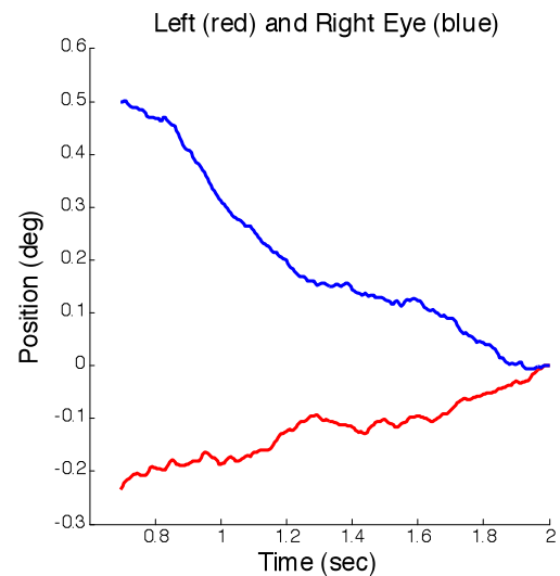
Figure 3 The fusion sustaining late portion of an individual response to a pure disparity vergence step stimulus plotted a version and vergence (upper plot) and as the actually recorded left and eye movements(lower plot).
