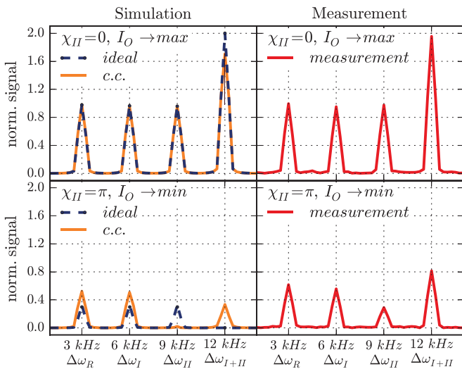
FIG. 3. Power spectra of simulations for perfect contrast (dashed blue line) and contrast corrected (solid orange line) are plotted on the left. Power spectra of the measurement (solid red line) are plotted on the right. The first row is obtained for the phase setting \chi_{II} = 0 , while the second row for the setting \chi_{II} = \pi .
