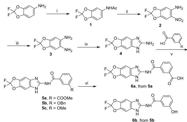
Scheme 1. Synthesis of reference standards 5a ; 5c and O -desmethylated precursors 6a ; 6b . Reaction reagents, conditions and yields: (i) acetic anhydride, toluene, 100 °C, 92%. (ii) NO 2 BF 4 , CH 2 Cl 2 , 69%. (iii) hydrogen, Pd/C, methanol; (iv) cyanogen bromide, methanol, room temperature (RT), 40 h, 82%. (v) 3-substituent-benzoic acid, HBTU, DIPEA, 18-63%. (vi) for 6a , KOH, methanol, 93%; for 6b , Me 2 S, BF 3 ·Et 2 O, CH 2 Cl 2 , 65%.
