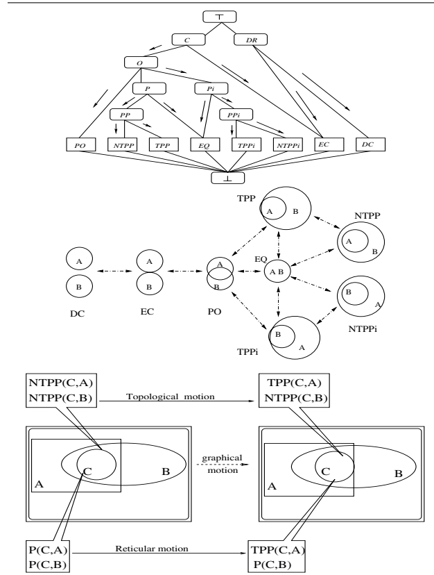
Figure 3. Reticular (up) and topological (down) motions in RCC8, and an example.
