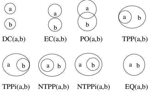
Figure 2. Axioms of RCC and RCC-8 relations
