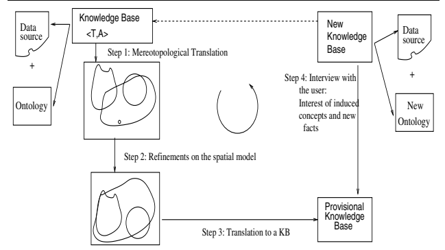
Figure 1. The ontology cleaning process
