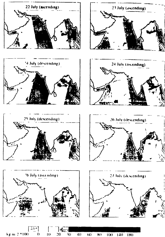
Figure 1. DMSI-SSM/I-derived cloud liquid water distribution for monsoon depression during 22–27 July, 1992
