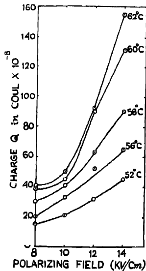
Fig. 3. Total heterocharge released to external circuit vs polarizing fields.
