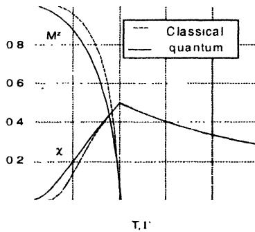
Figure 1. Variations of longitudinal sublattice magnetization and susceptibilities in the classical and quantum cases ( J = 1 ).
