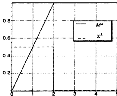
Figure 2. Variations of transverse magnetisation and susceptibility in the quantum case ( J = 1 ).
