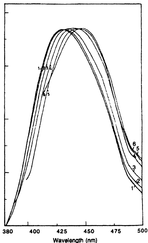
Figure 4. Excitation wavelength dependence of some peak-normalized emission spectra of 6MQ in Nafion ® film at 296K for \lambda_{ex} = 350 nm (1), \lambda_{ex} = 360 nm (2), \lambda_{ex} = 370 nm (3), \lambda_{ex} = 380 nm (4), \lambda_{ex} = 390 nm (5) and \lambda_{ex} = 400 nm (6).
