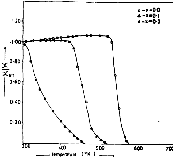
Figure 3. Variation of susceptibility with temperature for Mg_{0.7+r}Zn_{0.3}Sn_xFe_{2-2r}O_4 system.
