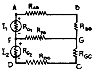
Fig. 1. Diagram for D.C. three wire Transmission-Network.
