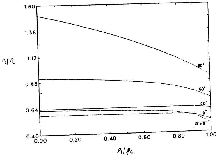
Figure 2. The behaviour of the plasma densities on either side of the density discontinuity plotted as a function of \theta for \gamma_1 = 70^\circ , \gamma_2 = 60^\circ
