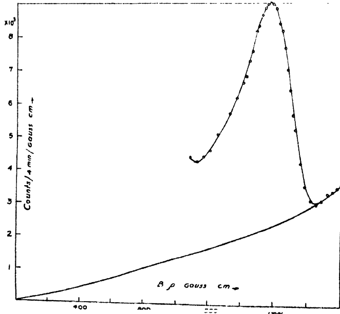
Fig. 2. Beta spectrum of In-114m source translated into momentum distribution. The recorded spectrum is represented by \bullet and the continuous line is the extrapolation to the origin.
