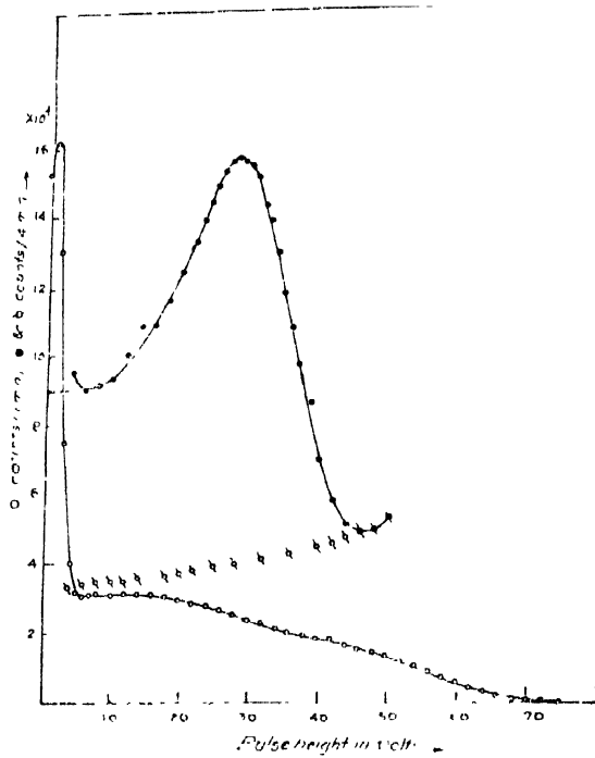
Fig. 1. Beta and conversion electron spectra of In-114m source. The points o represent the total spectrum for low gain of the amplifier. The points \bullet represent the conversion electrons at high gain. The points \circ represent the extrapolated beta spectrum obtained from Fig. 2.
