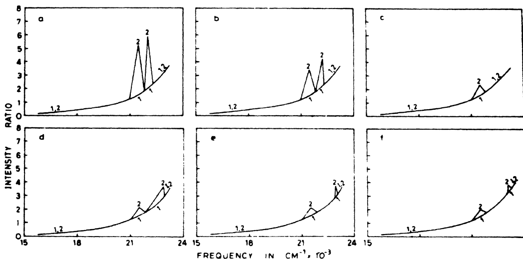
Figure 1. Calculated Raman excitation profiles of some totally symmetric vibrations of quinoxaline a 532 \text{cm}^{-1} b 758 \text{cm}^{-1} c 1204 \text{cm}^{-1} d 1367 \text{cm}^{-1} e 1415 \text{cm}^{-1} and f 1570 \text{cm}^{-1}
