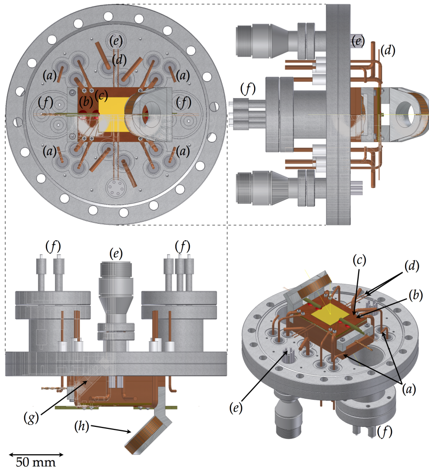
Figure 3.4: Layout of the atom chip flange that sits on top of the chamber. It features electrical feedthroughs for the quadrupole coils ( a ) that form the MOT, the end wire structures ( b ), the H-structure (partly covered by the waveguide chip) ( c ), the atom chip bias field wires ( d ), dispensers (only the feedthroughs shown here) ( e ). In addition, there are optical feedthroughs ( f ) to bring light to the waveguide chip. The side cross section view of the flange also shows that one of the quadrupole coils is embedded into the copper block ( g ), another is mounted on an aluminium support ( h ).
