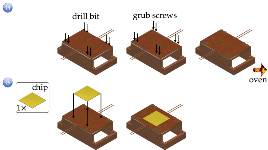
Figure 4.8: Manufacturing process: steps (14) and (15).
