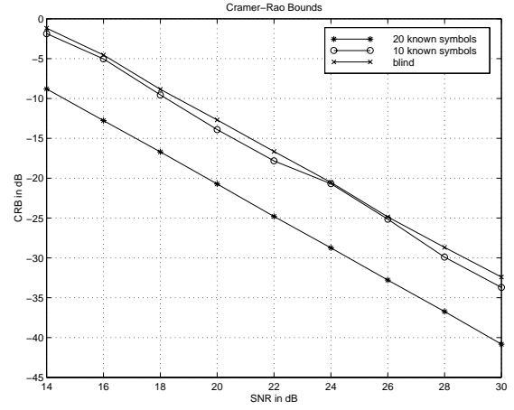
Figure 3: CRB's of blind and semi-blind DML
