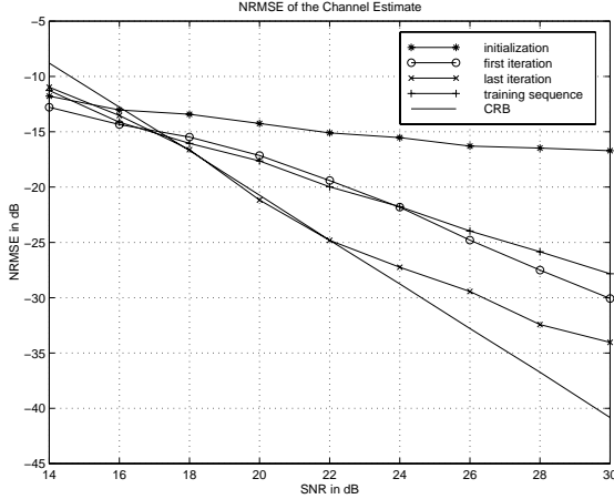
Figure 2: Performance of semi-blind PQDML
