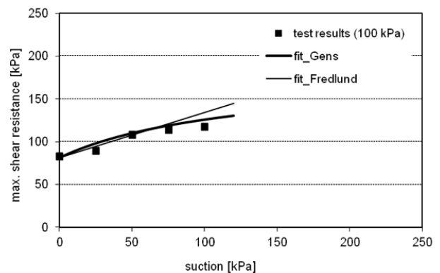
Figure 20. Tössegg: Shear strength envelopes for suction-controlled direct shear tests on silty sand with peak shear stress mobilised as a function of suction [after 58].
