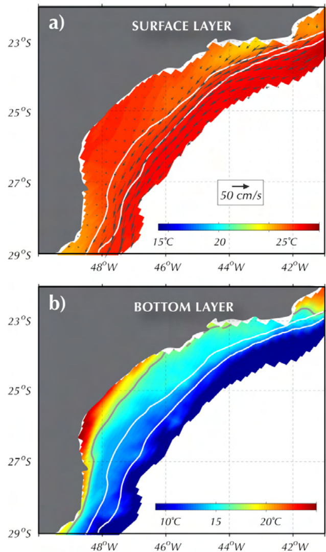
Fig. 4. EXP2: (a) Summer sea surface temperature and surface velocity vectors and (b) Bottom temperature. White contours mark the 100 and 200 isobaths. The black line in panel (b) is the 17 °C isotherm, indicative of the SACW penetration. Note that each panel uses a different color bar.
