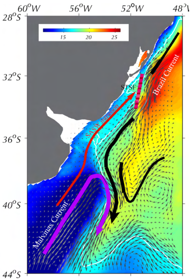
Fig. 13. Snapshot of SST and velocities in EXP1. This figure shows a classic configuration of the circulation in this region, which is characterized by the detrainment of shelf waters onto the deep ocean.
