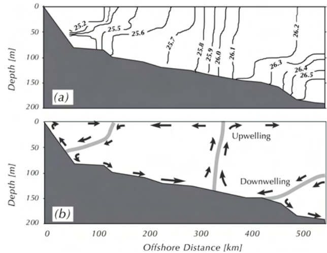
Fig. 11. Density cross-shelf section off Grande Bay ( \sim 51^{\circ} S) from a hydrographic cruise in March 1994 (top panel). Schematic showing the fronts identified in this section and the inferred circulation patterns. (After Sabatini et al., 2004).
