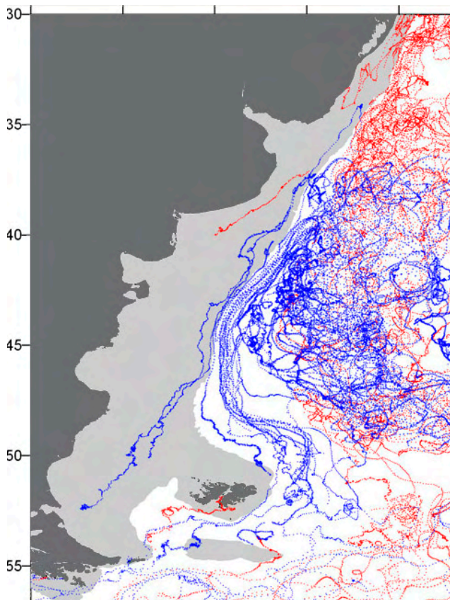
Fig. 14. Trajectories of satellite tracked “surface” drifters from WOCE-Surface Velocity Program type. The drifters are drogued to 15 m depth and designed to follow the water to within \pm 0.13 \text{ m s}^{-1} in 10 \text{ m s}^{-1} winds (Niiler et al., 1995). The original position data have been quality controlled and optimally interpolated to uniform six-hour interval trajectories (Hansen and Poulain, 1996). Note the quasi-linear trajectories of the drifters in the MC.
