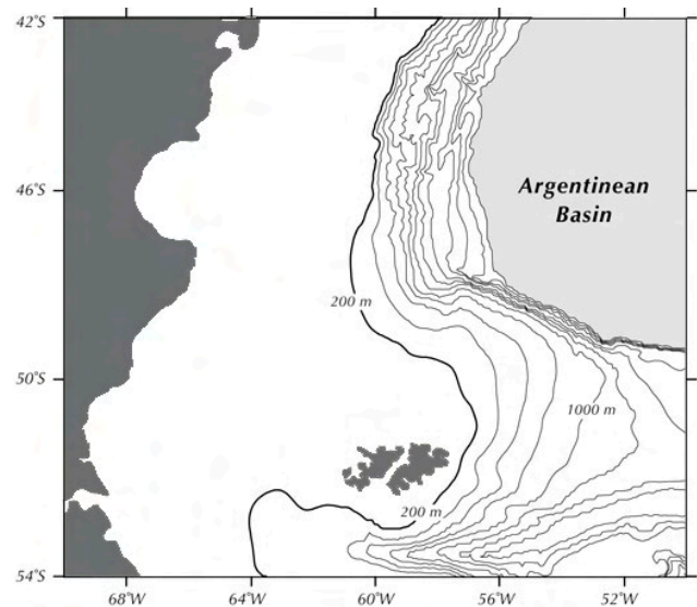
Fig. 15. Bottom topography of the Patagonian shelf. Note the rapid convergence of the isobaths north of \sim 50^\circ \text{ S} .
