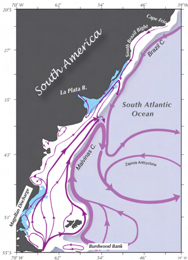
Fig. 1. Schematic representation of the depth-averaged circulation in the southwestern Atlantic region. The shelf (depths smaller than 200 m) is marked by white background.
