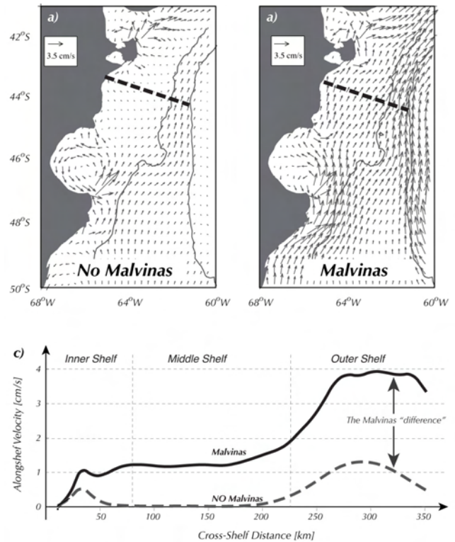
Fig. 9. (a) Depth averaged velocities in EXP2; (b) EXP1; (c) Alongshelf velocities across the section shown in the upper panels. The differences between these two experiments are mainly due to the MC.
