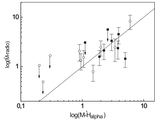
Fig. 13. H\alpha -derived versus radio-derived mass-loss rates. Units are 10^{-6} M_{\odot} \text{yr}^{-1} . Squares: stars above the BSJ temperature; open circles: stars below the jump temperature. Symbols with arrows represent upper limits in \dot{M}_{\text{radio}} .
