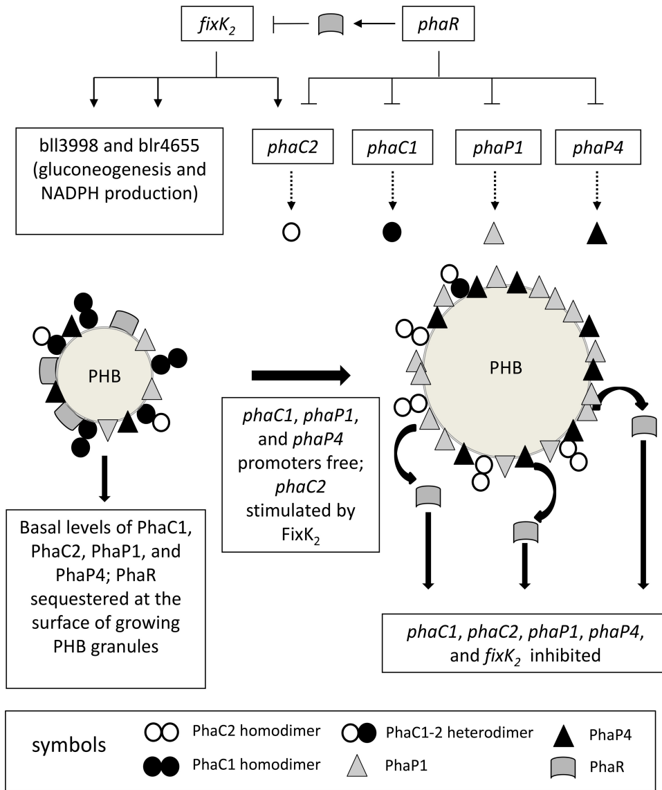
FIG 5 Proposed model for the regulation of PHB synthesis in B. diazoefficiens , including the possible role of FixK2 (→, stimulation; ⊥, inhibition; solid lines indicate transcription; dashed lines depict translation). Permissive conditions, e.g., low O_2 , lead to an increase of NADPH and acetyl-CoA concentrations; thus, PHB biosynthesis starts using these metabolites as the substrates. This biosynthetic process is catalyzed initially by high levels of 3-ketoacyl-CoA thiolase, acetoacetyl-CoA reductase, and PHB synthase due to PhaR sequestration at the PHB granule surface. Meanwhile, phaC2 expression is stimulated by FixK2 , increasing the relative PhaC2/PhaC1 concentration, which progressively decreases total PhaC activity during PHB granule growth. As granules grow, less PHB surface becomes available for PhaR and PhaP, which may provoke a competitive displacement of PhaR by PhaP from the surface that in turn may repress PhaR-controlled promoters. In the phaR mutant, these promoters are not repressed; therefore, PhaP1, PhaP4, and FixK2 levels are increased. Hence, FixK2 stimulates the expression of phaC2 and the biosynthesis of EPS. Altogether, these changes result in low levels of PHB in the phaR mutant. Moreover, in the \Delta phaP1 \Delta phaP4 strain, the very large PHB granule devoid of PhaP1 and PhaP4 may be able to allocate more PhaR than the wild type at the beginning of PHB biosynthesis. This PhaR sequestration may promote more PHB biosynthetic activity, leading to higher PHB accumulation before the PhaC2/PhaC1 ratio reaches its critical value and PhaR begins to accumulate in the cytoplasm. Protein symbols are indicated at the bottom of the figure. For more details, see the text.
