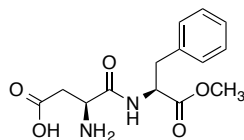
Figure 1: Aspartame molecular structure.
