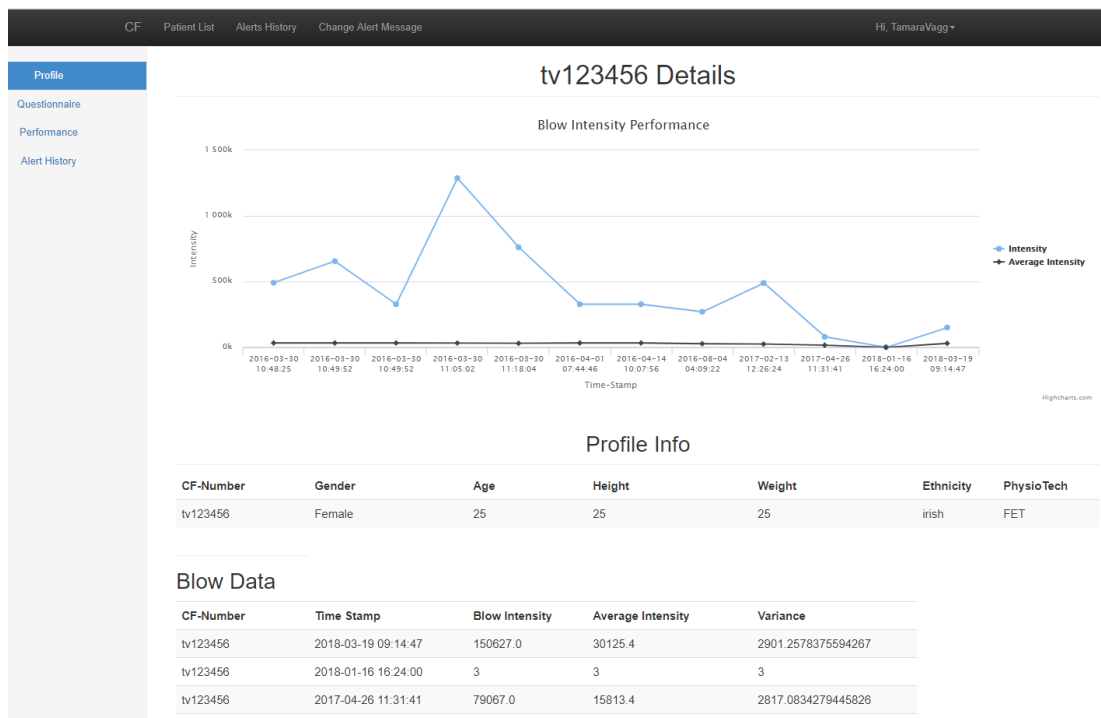
Figure 5.7: A screenshot of the web tool showing patient calibration data. Further screenshots in Appendix E.
