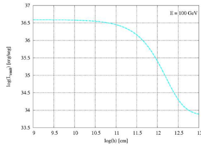
Figure 4. Intrinsic luminosity L_{emit} as a function of h .
