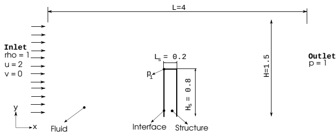
Fig. 3. Fluid domain and dimensions.
