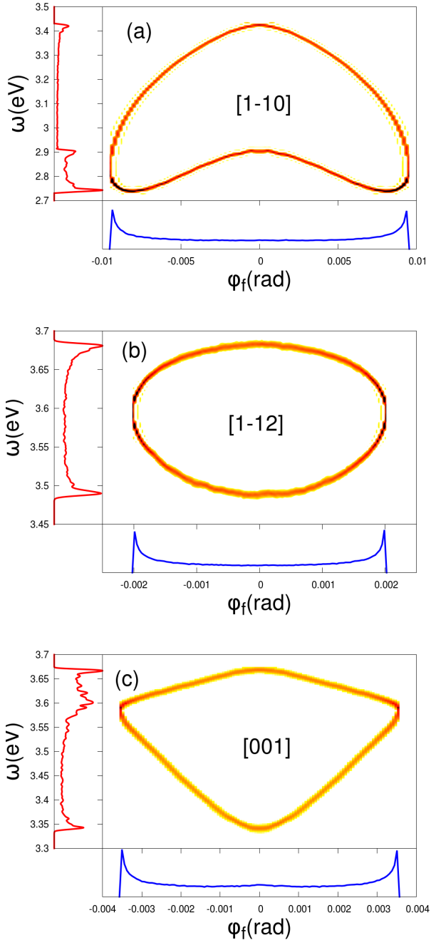
FIG. 5: (Color online) 2D angle- and energy-loss distributions, as a function of the final azimuthal angle \varphi_f and the lost energy \omega , for 1 keV He atoms impinging on Ag(110) with \theta_i = 1^\circ . Three different incidence directions are considered: (a) [1\bar{1}0] , (b) [1\bar{1}2] , and (c) [001] . Integrated angular and energy-loss spectra are also shown in the figure.
