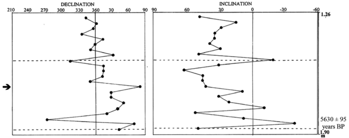
Figure 8. Stratigraphic plots of the declination and inclination profiles from Mu. The more conspicuous long direction and inclination departures are depicted between dashed lines and pointed with an arrow.
