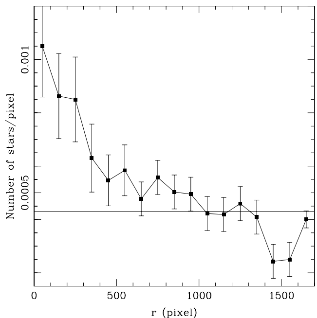
Figure 4. Stellar density profile centred at (x_c, y_c) = (1200, 1200) pixels for stars observed in the field of NGC 2489. The horizontal line represents the background level measured for r > 1000 pixels.
