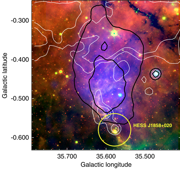
Fig. 1. Three color image of the analyzed region (red=8 \mu\text{m} , green = 24 \mu\text{m} , and blue = 20 cm radio continuum emission). The black contours delineate the radio continuum emission with levels of 20 and 28 K. The white contours are the ^{13}\text{CO } J = 1-0 emission integrated between 51 and 59 \text{km s}^{-1} , its levels are 3.2 and 5 \text{K km s}^{-1} . The yellow circle represents the source HESS J1858+020.
