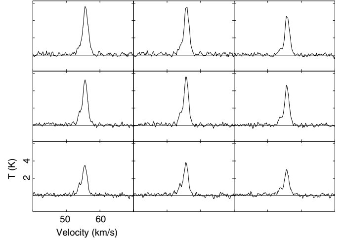
Fig. 2. ^{13}\text{CO } J = 1-0 spectra obtained towards the maximum of the molecular clump that lies over the SNR shell. The spectra, which show brightness temperature vs. velocity, correspond to nine positions observed in a region of about 50'' \times 50'' centered at the molecular clump peak.
