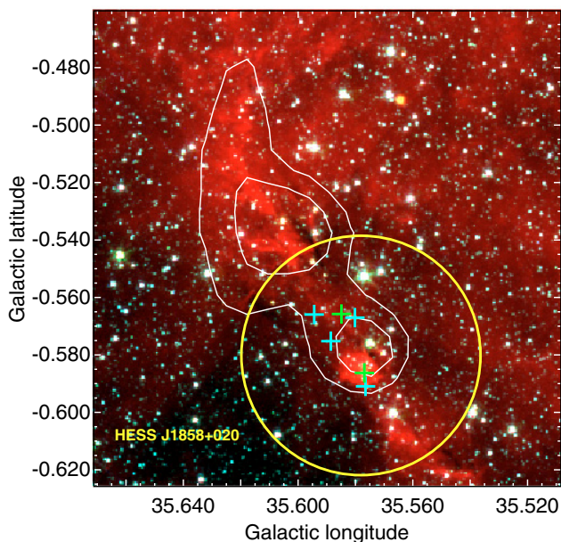
Fig. 3. Three color image of IRAC- Spitzer bands (red = 8 \mu\text{m} , green = 4.5 \mu\text{m} , and blue = 3.6 \mu\text{m} ). The white contours are the ^{13}\text{CO} J = 1-0 emission integrated between 51 and 59 \text{km s}^{-1} , its levels are 3.2 and 5 \text{K km s}^{-1} . The crosses are YSO candidates according to the photometric study described in the text. Green crosses are Class I sources and cyan crosses represent Class II sources.
