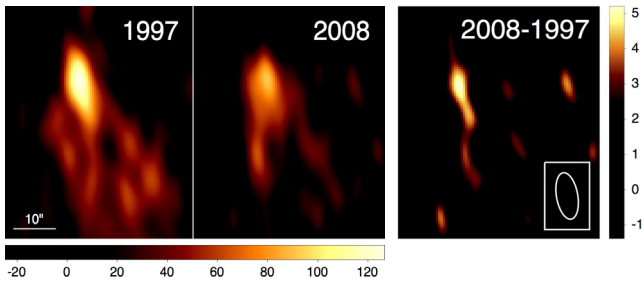
Fig. 2. Close up of the northern radio lobe of GRS 1758–258 as observed with the VLA at 6 cm in 1997 ( left ) and 2008 ( middle ), when the hotspot was fainter. The coloured horizontal bar provides a linear intensity scale in \mu\text{Jy beam}^{-1} . The bottom left corner bar gives the angular scale. North is up and east left. The right panel shows the residual difference between the two epochs. Its colour vertical bar is scaled in units of the rms noise in the difference map ( 10 \mu\text{Jy beam}^{-1} ). The synthesized beam in all panels is the same as in Fig. 1 (bottom right ellipse).
