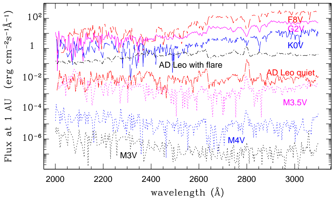
Fig. 1. Buccino et al. , 2007. IUE spectra of M stars.
