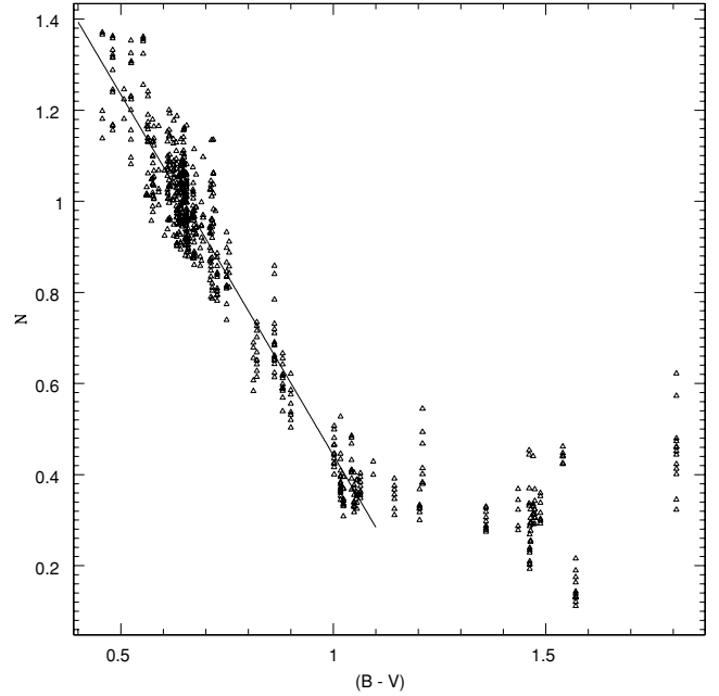
Figure 8. N index versus colour index (B - V) . The solid line is the best linear fit for stars with (B - V) < 1.1 . Stars with a larger (B - V) do not show any correlation.
