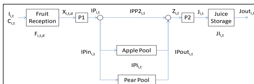
Figure 1 – Pome fruit juice plant process flowsheet
