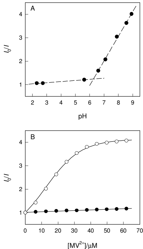
Fig. 4. Quenching of the emission at 595 nm of Ru(bpy) 3 @SiO 2 NPs by MV 2+ as a function of pH (A) and MV 2+ concentration (B); in A, [MV 2+ ] = 62 \mu\text{M} ; in B, pH 3.0 (●), pH 8.9 (○).
