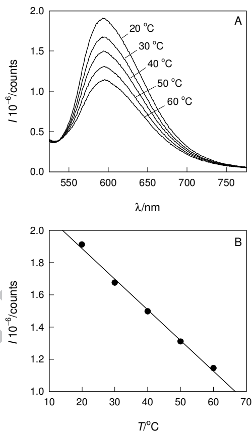
Fig. 5. Emission spectra of \text{Ru}(\text{bpy})_3@ \text{SiO}_2 NPs (A), and emission at 595 nm (B) as a function of temperature; \lambda_{\text{exc}} = 463 nm; slit = 1.6 mm.
