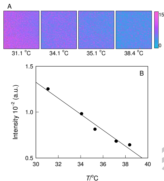
Fig. 7. 20 \times 20 \mu\text{m} SCM images of \text{Ru}(\text{bpy})_3@/\text{SiO}_2 NPs adhered to PEI-modified glass (A), and mean fluorescence intensity as a function of temperature (B).
