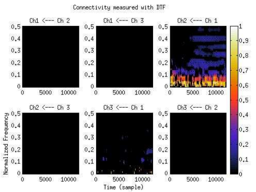
Figure 9. DTF for APP-ML simulation. A \rightarrow P1 show effective connectivity mainly in the lower frequency band. P1 \rightarrow P2 connectivity not detected. Indirect connectivity is measured between A \rightarrow P2 . Ch 1: A population, Ch 2: P1 population, Ch 3: P2 population.
