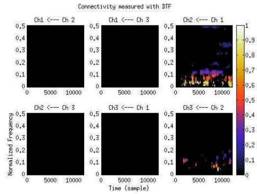
Figure 7. DTF for APP-MM simulation. A \rightarrow P1 and P1 \rightarrow P2 show effective connectivity in the lower frequency band. P1 \rightarrow P2 connectivity shows lower strength. Ch 1: A population, Ch 2: P1 population, Ch 3: P2 population.
