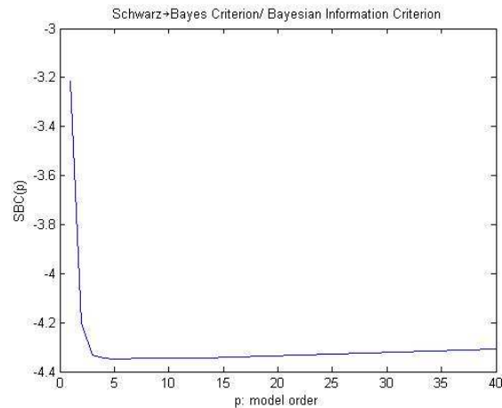
Figure 3. Bayesian criterion shows that the chosen model order is acceptable
