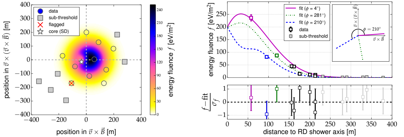
FIG. 3. Lateral signal distribution of a single cosmic-ray event. The air-shower properties of this event are: Energy of 0.75 EeV and arriving at a zenith angle of 37^\circ and from 44^\circ west of south. Left: The energy fluence in the shower plane. The measurements are indicated as circles where the color shows the energy fluence. Gray squares are stations with signal below threshold and the red cross marks a station that is rejected due to a mismatch in the signal polarization. The background map shows the LDF parametrization. The coordinate origin is the reconstructed core position of the radio LDF fit. Note the lack of color contrast between the infill color of the data points and the background. This is indicative of the agreement between the data and the model. Right: Representation of the same data as a function of distance from the shower axis. The colored and black squares are the measured energy fluences and gray squares are the stations with signal below threshold. For the three data points with the highest energy fluence, the one-dimensional projection of the two-dimensional LDF onto lines connecting the radio-core position with the corresponding radio detector positions is illustrated with colored lines. This demonstrates the azimuthal asymmetry and complexity of the two-dimensional lateral distribution function. The inset figure shows the azimuthal direction of the three LDF projections. The distribution of the residuals (data versus fit) is shown as well.
