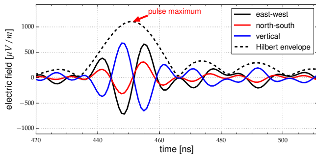
FIG. 1. Reconstructed electric-field trace of one of the measured cosmic-ray radio events. An upsampling by a factor of five was applied. The shown Hilbert envelope (dashed line) is the square root of the quadratic sum of the Hilbert envelopes of the three polarization components.
