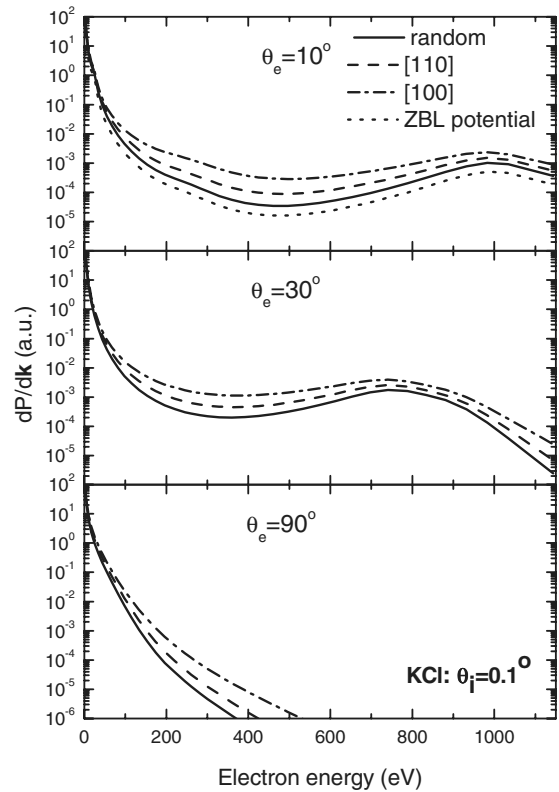
FIG. 3. Similar to Fig. 1 for protons impinging on a KCl (001) surface with the incidence angle \theta_i=0.1^\circ .
