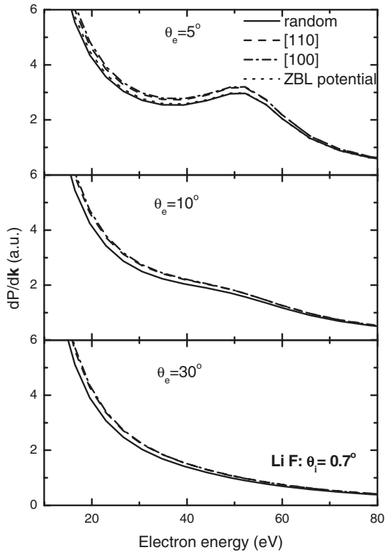
FIG. 2. Similar to Fig. 1 for the incidence angle \theta_i=0.7^\circ .
