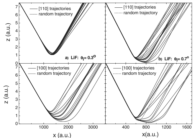
FIG. 4. Random set of trajectories corresponding to the results of (a) Fig. 1 (left two graphs) and (b) Fig. 2 (right two graphs).
