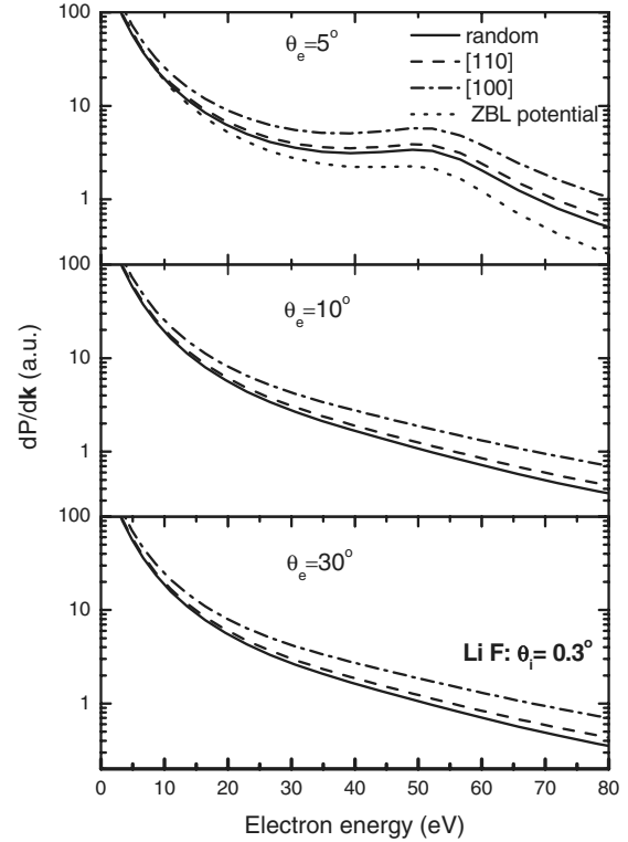
FIG. 1. Emission probability for electrons ejected from a \text{LiF} (001) surface at the emission angles \theta_e = 5, 10, and 30^\circ , as a function of the electron energy. The incidence angle is \theta_i = 0.3^\circ . Three incidence directions of protons are considered. Full line, random incidence corresponds to a polar angle far from low-index crystallographic orientations; dashed and dashed-dotted lines correspond to the directions of the two principal axes, [110] and [100], as indicated in the figure. Dotted line, results obtained by using a planar ZBL potential to derive the projectile trajectory.
