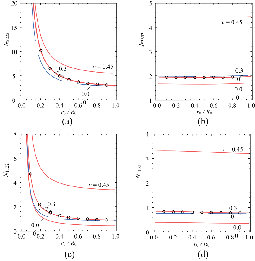
Figure 12. Normalized nonzero components of the stiffness contribution tensor of inhomogeneity (a) N_{1111} = N_{2222} , (b) N_{3333} , (c) N_{1122} , (d) N_{1133} , (e) N_{1212} , and (f) N_{1313} = N_{2323} as function of the aspect ratio r_0/R_0 . The solid curves correspond to the rigid toroidal inclusion; The dashed curves correspond to the rigid ellipsoidal inclusion; the FEM results are noted by marks. The stiffness values are given in units of \epsilon_{ij}E for different values of Poisson ratio 0.0, 0.3, and 0.45.
