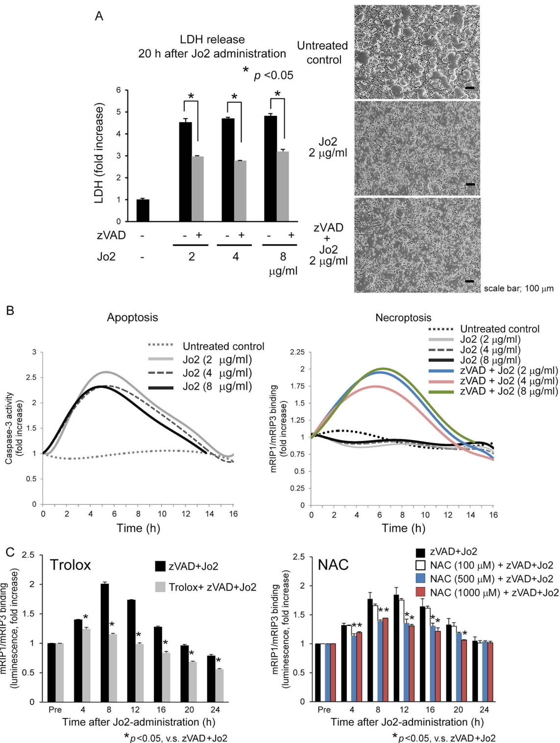
Figure 3. Fas ligand (FasL; Jo2) induced necrotic cell death and RIP1/3 binding in a redox-dependent manner in TIB-73 cells. (A) A caspase inhibitor (zVAD) only partially suppressed FasL (Jo2)-induced necrotic cell death in TIB-73 cells. (B) Optic probes for caspase 3 activity (left) and RIP1/3 binding (right) were used to evaluate apoptosis and necroptosis, respectively. FasL (Jo2) induced activation of caspase 3, and RIP1/3 binding occurred only when the caspases were inactivated. (C) Antioxidants [Trolox and N -acetyl cysteine (NAC)] significantly suppressed FasL (Jo2; 2 µg/ml)-induced RIP1/3 binding. The concentration of zVAD used was 20 µM (A, B, and C). Results are expressed as mean \pm SEM of five independent experiments, with p < 0.05 considered significant (A, C). Data from the optic probes and photomicrographs are representative of at least three independent experiments.
