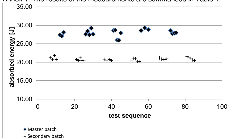
Figure 3: Absorbed energy values of 29 test pieces of ERM ® -FA013br, compared with 20 test pieces of ERM ® -FA013ba; data are displayed in the actual test sequence.
